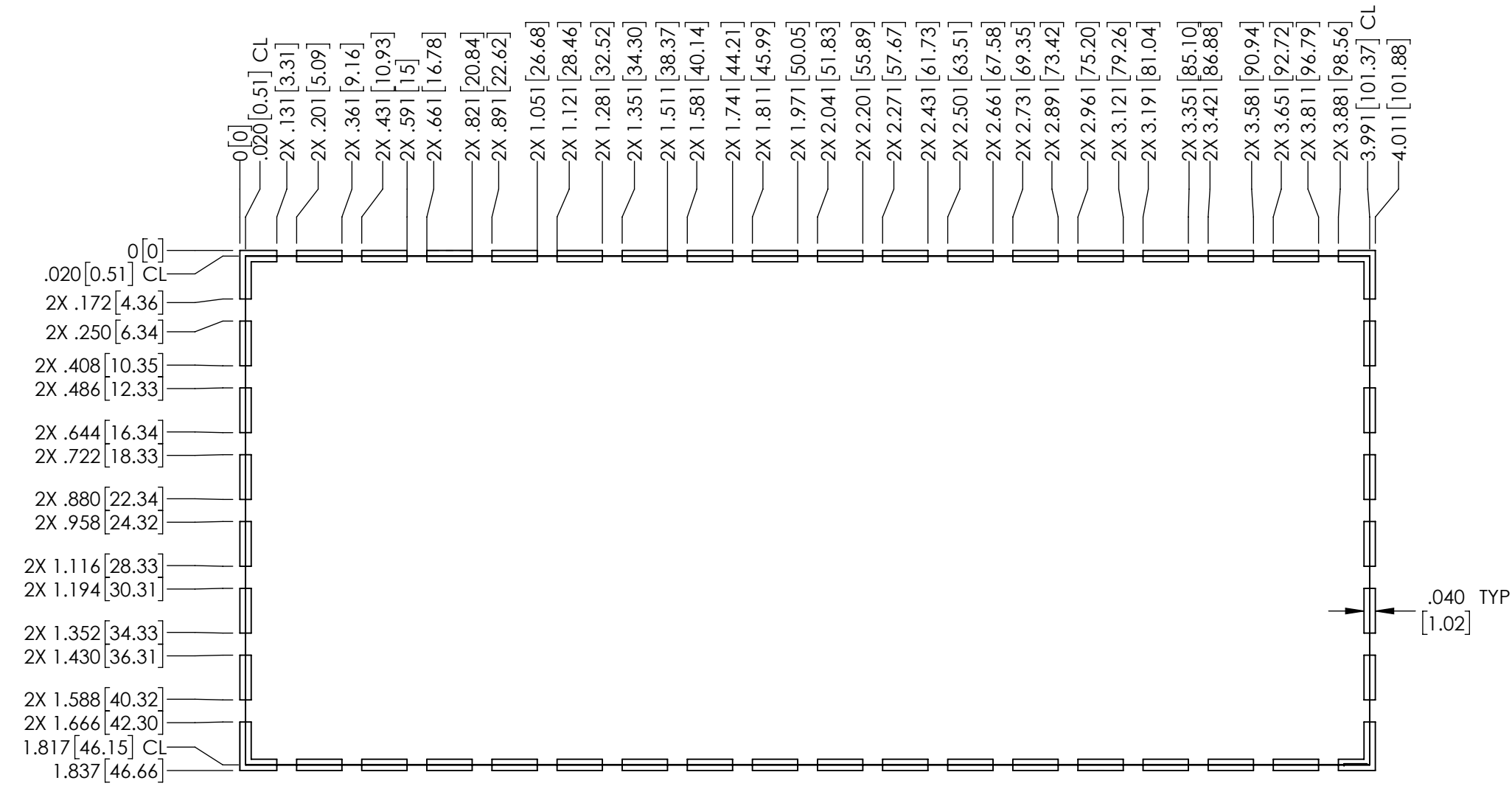
TRACE PATTERN
