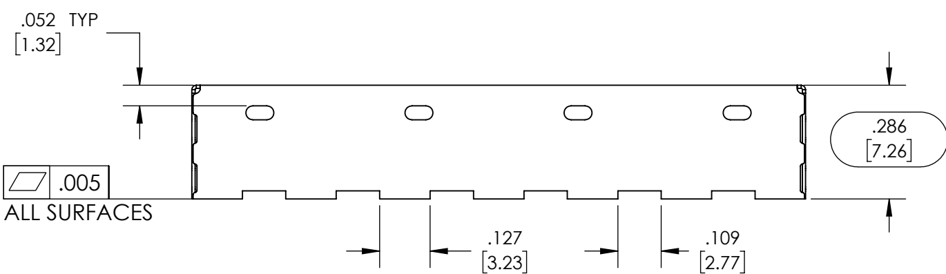
FORMED FRAME
