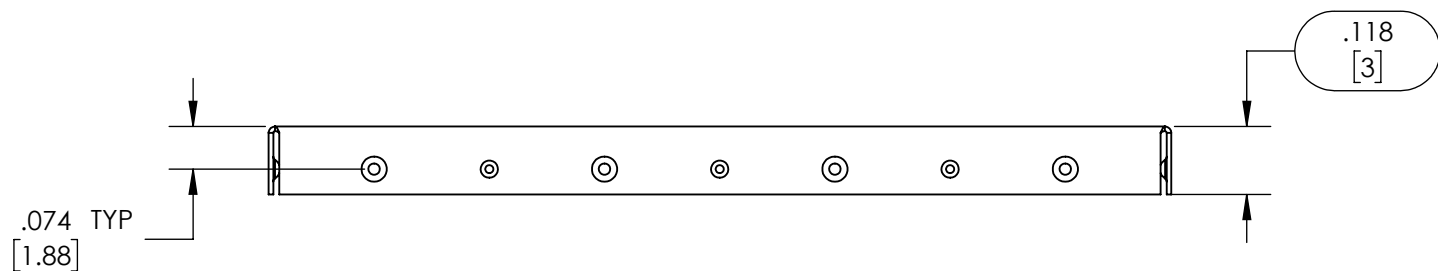
FORMED COVER
