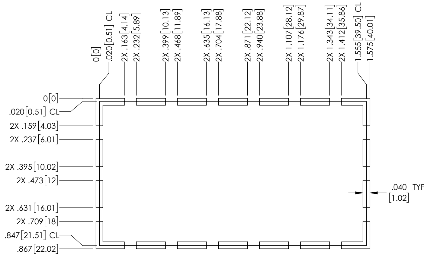
TRACE PATTERN
