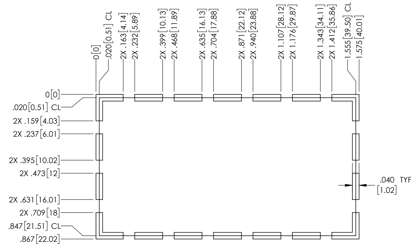
TRACE PATTERN
