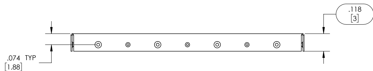
FORMED COVER
