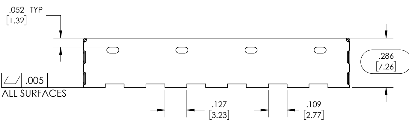
FORMED FRAME
