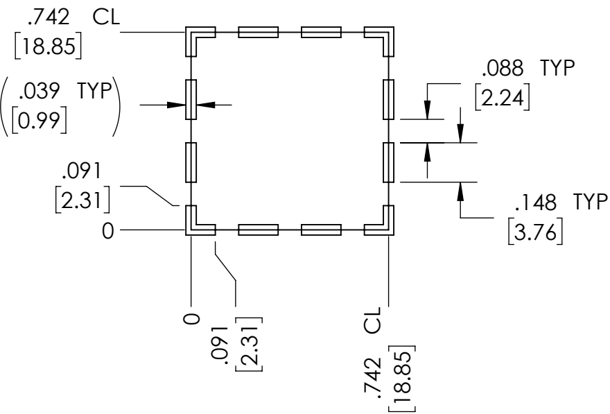
TRACE PATTERN
