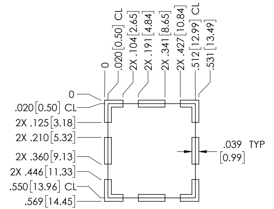
TRACE PATTERN
