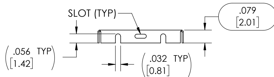
FORMED COVER
