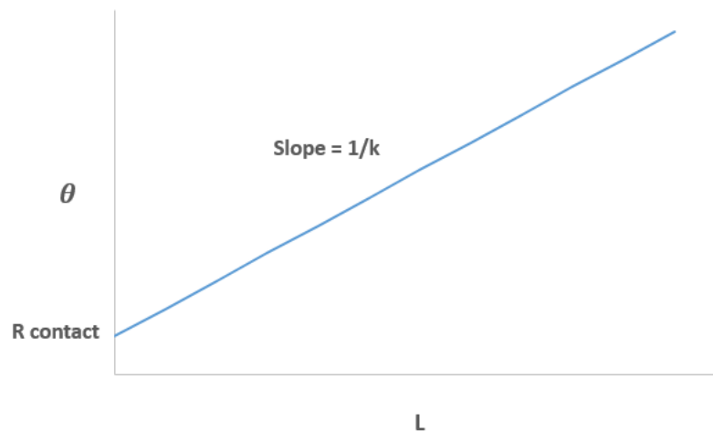
Figure #2. Thermal Impedance vs Thickness
