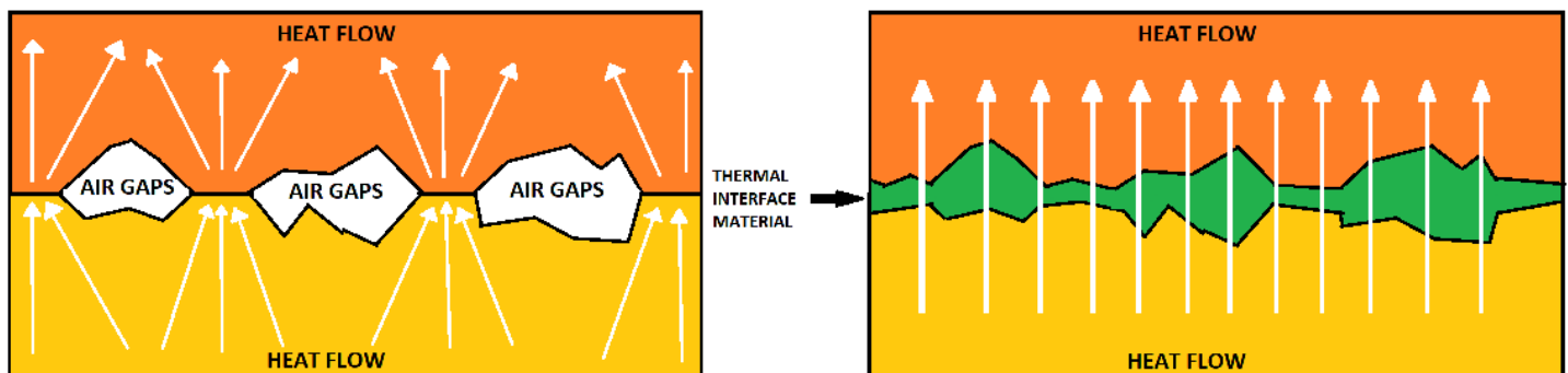
Figure #1. Two surfaces in contact and heat flowing across the surfaces without (left) and with thermal interface material (right).
