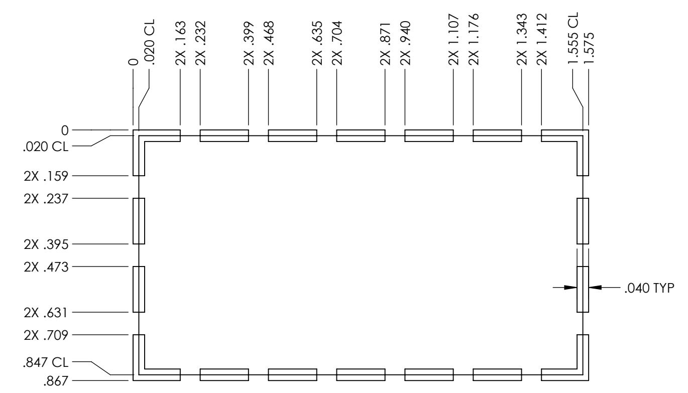
TRACE PATTERN
