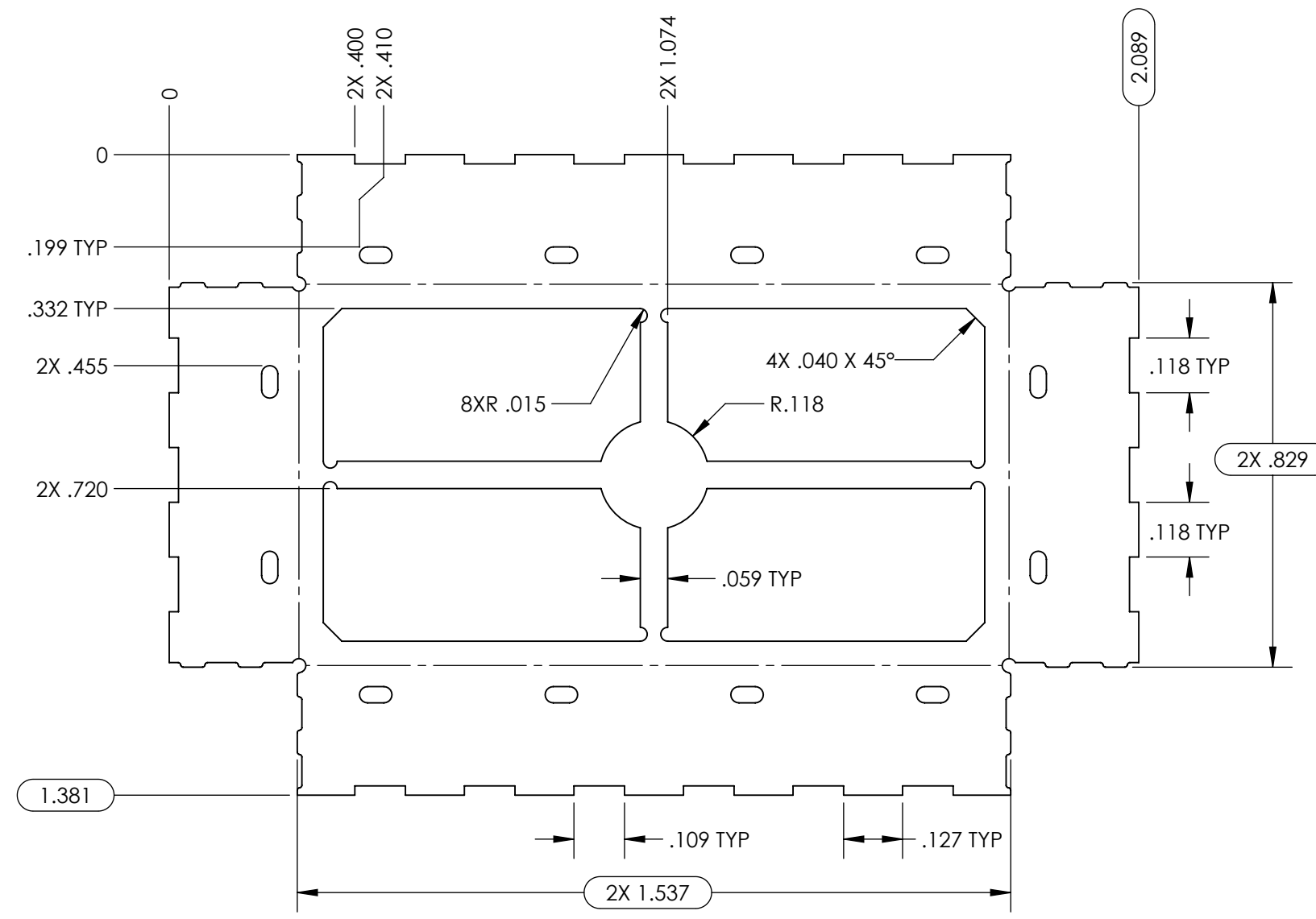
FRAME BLANK
