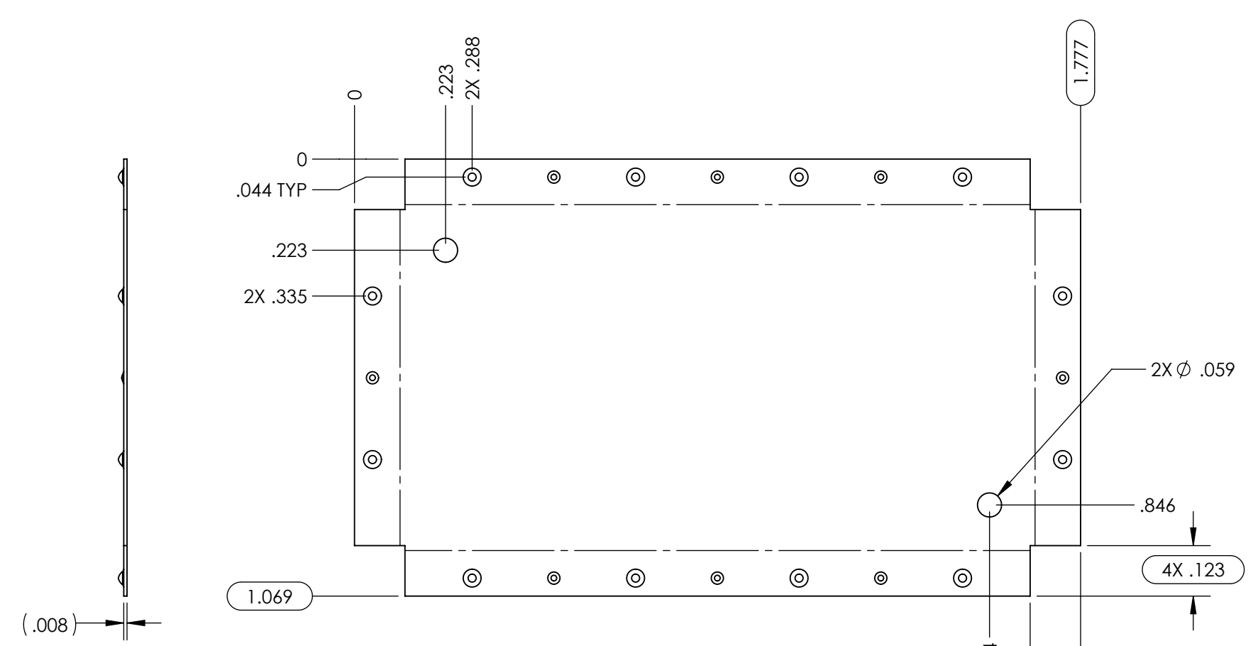
COVER BLANK
